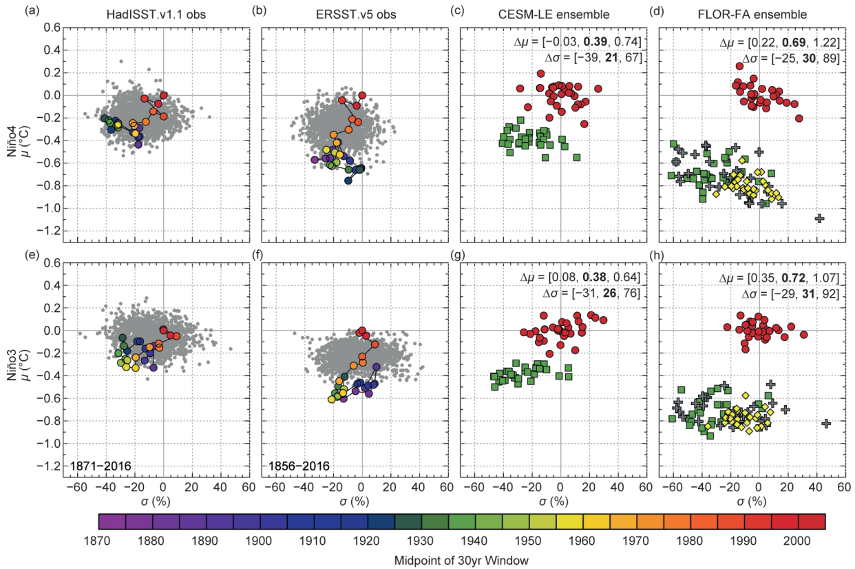
FIG. 4.2. Statistics for annually smoothed SSTs averaged over (a)–(d) Niño4 and (e)–(h) Niño3. Y-axis is the 30-year mean ( \mu , °C departure from 1871–2016); x-axis is the 30-year std dev ( \sigma , % departure from 1871–2016). (a),(b),(e),(f) sample the observationally reconstructed 30-year statistics every 5 years (colored dots). Gray dots show analogous statistics from 8000-year LIM simulations trained using detrended 1959–2000 data from HadISST.v1.1 or ERSST.v5. (c),(g) show the CESM-LE 30-member ensemble simulation with “ALL” (anthropogenic + natural) historical forcings, for 1987–2016 (red dots) and 1920–49 (green squares) relative to the 1987–2016 ensemble mean; inset indicates ALL ensemble [minimum, average, maximum] change in \mu and \sigma from 1920–49 to 1871–2016. (d),(h) show analogous statistics for the FLOR-FA 30-member ALL ensemble, along with a 30-member “NAT” ensemble with natural forcings only for 1920–49 (gray crosses) and 1987–2016 (yellow diamonds), also relative to the ALL ensemble mean.
