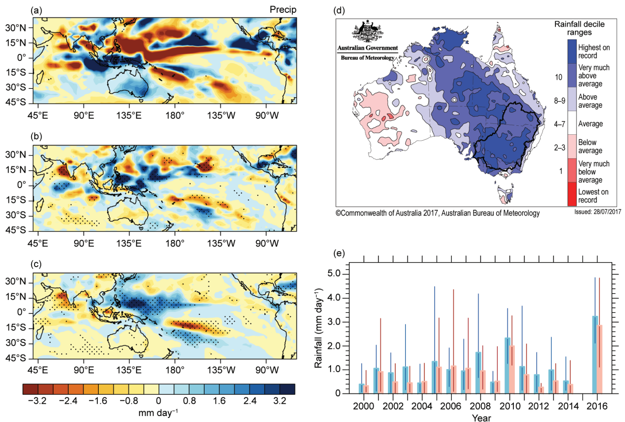
FIG. 26.1. (a) Forecast rainfall anomaly (mm day -1 ) from 2000–14 climatology) for 15–28 Sep 2016, using 11 members of model version a. (b) Difference between 2016 forecast rainfall (mm day -1 ) under current levels of CO 2 (401.03 ppm; www.esrl.noaa.gov/gmd/ccgg/trends/data.html ) and 1960 CO 2 levels (315 ppm), using 11 members of model versions a,b,c (33 total). (c) Climatological rainfall difference (mm day -1 ) for current minus low CO 2 levels, using 11 members of model version a. Stippling in (b) and (c) indicates significant differences (10% level). (d) Outline of MDB region, over rainfall deciles for Sep 2016 (relative to 1901–2016), and (e) ensemble mean rainfall forecast (mm day -1 ) time series for last two weeks of Sep under current (red bars) and low CO 2 (blue bars) conditions for MDB region. Lines show ensemble spread across 11 members.
