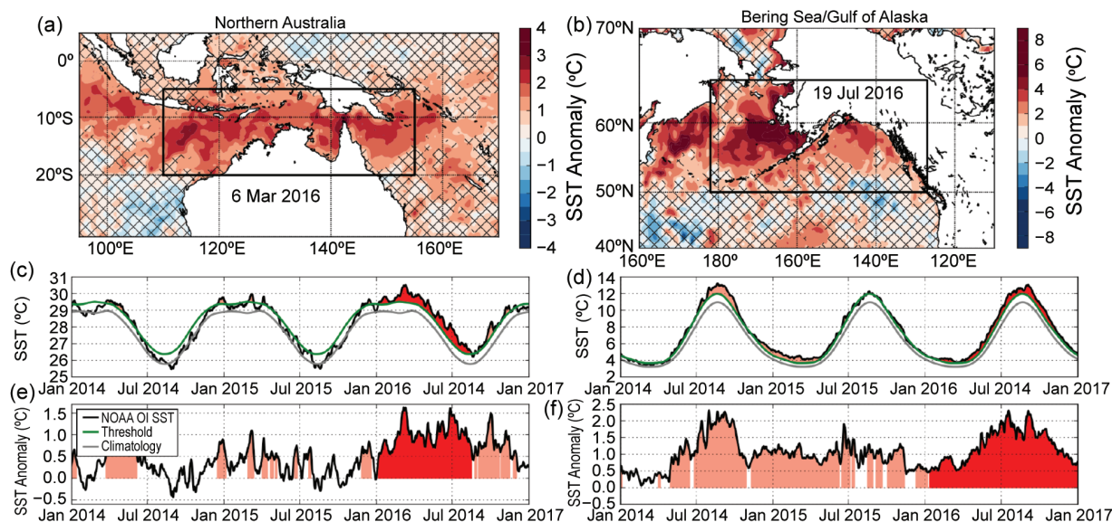
FIG. 9.1. 2016 MHWs in (left) NA and (right) BSGA. (a),(b) SST anomalies (°C) during the peak of each event (date indicated in panel) and unhatched areas indicate regions defined as MHW on that date according to the Hobday et al. (2016) definition. (c),(d) Daily SSTs (°C): NOAA OI SST (black), threshold (green), and 1961–90 climatology (gray) (e),(f) SST anomalies (°C) averaged over NA and BSGA during 2014–16. In (c)–(f) red shading indicates the 2016 MHW; lighter shading indicates other detected marine heat waves over the period.
